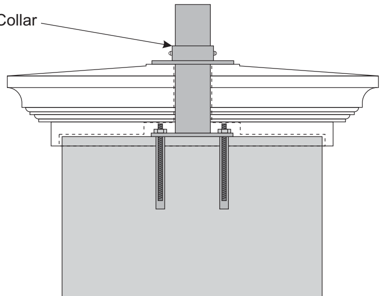
Recessed Mount
