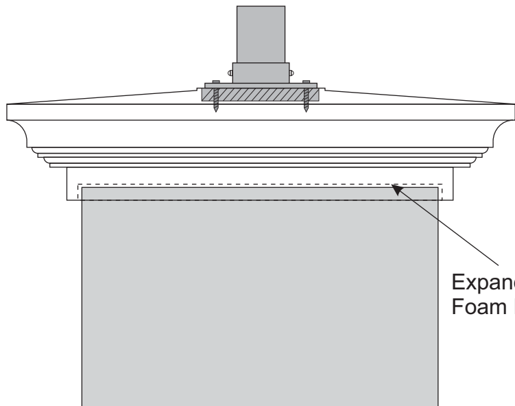
Flush Mount
